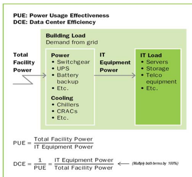
Figure 1: Illustration of How PUE and DCE Would Be Calculated In A Datacenter
